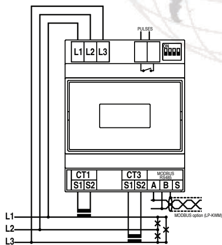
LP-2KW3C/M - 3-phase 3 wire unbalanced load
