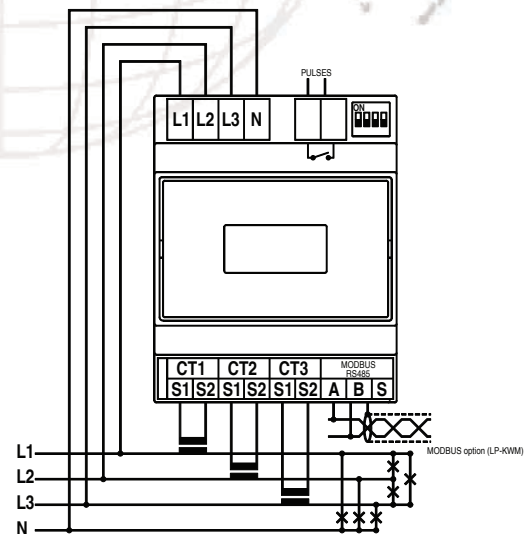
LP-3KW4C/M - 3-phase 4 wire unbalanced load
