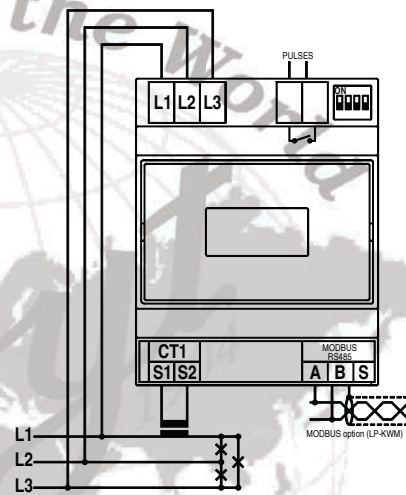
LP-1KW3C/M - 3-phase 3 wire balanced load
