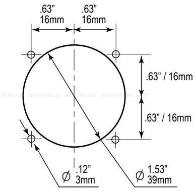
PANEL CUT-OUT
